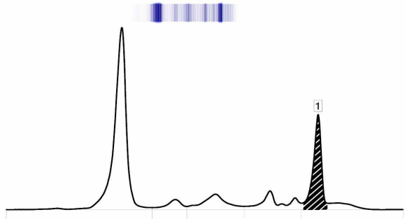
Electrophoresis Image
